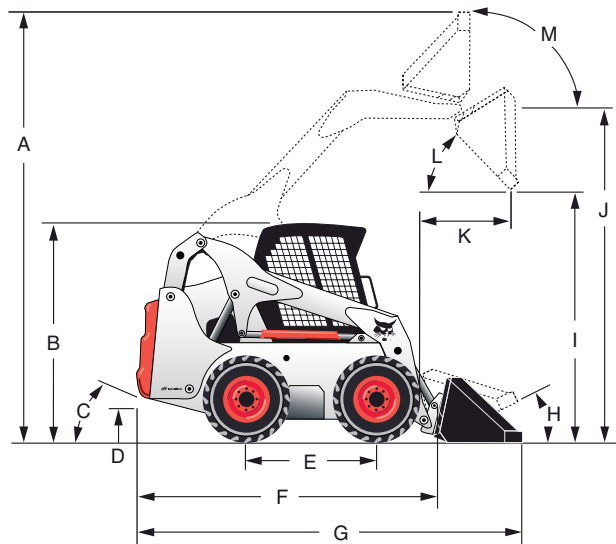
Vertical lift path: S250(H), S300(H), A300(H)
